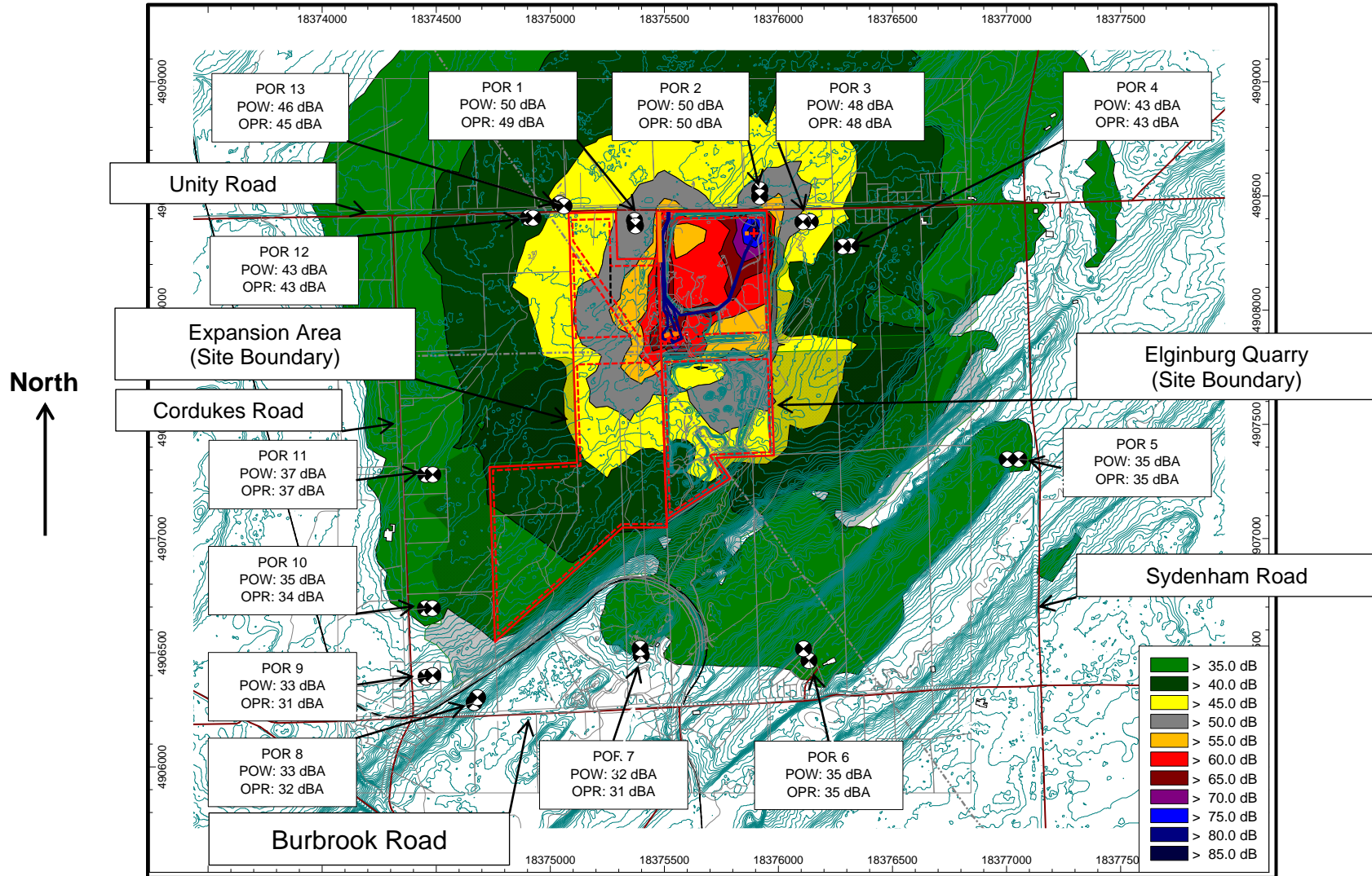
Figure 4.2: Scenario 1: Worst Case – Noise Contours, Day Only: (Noise levels at 4.5 m) – After Mitigation
