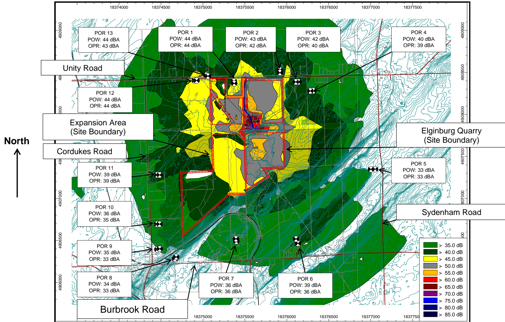
Figure 22.2: Scenario 10: Worst Case – Noise Contours, Night: (Noise levels at 4.5 m) – After Mitigation
