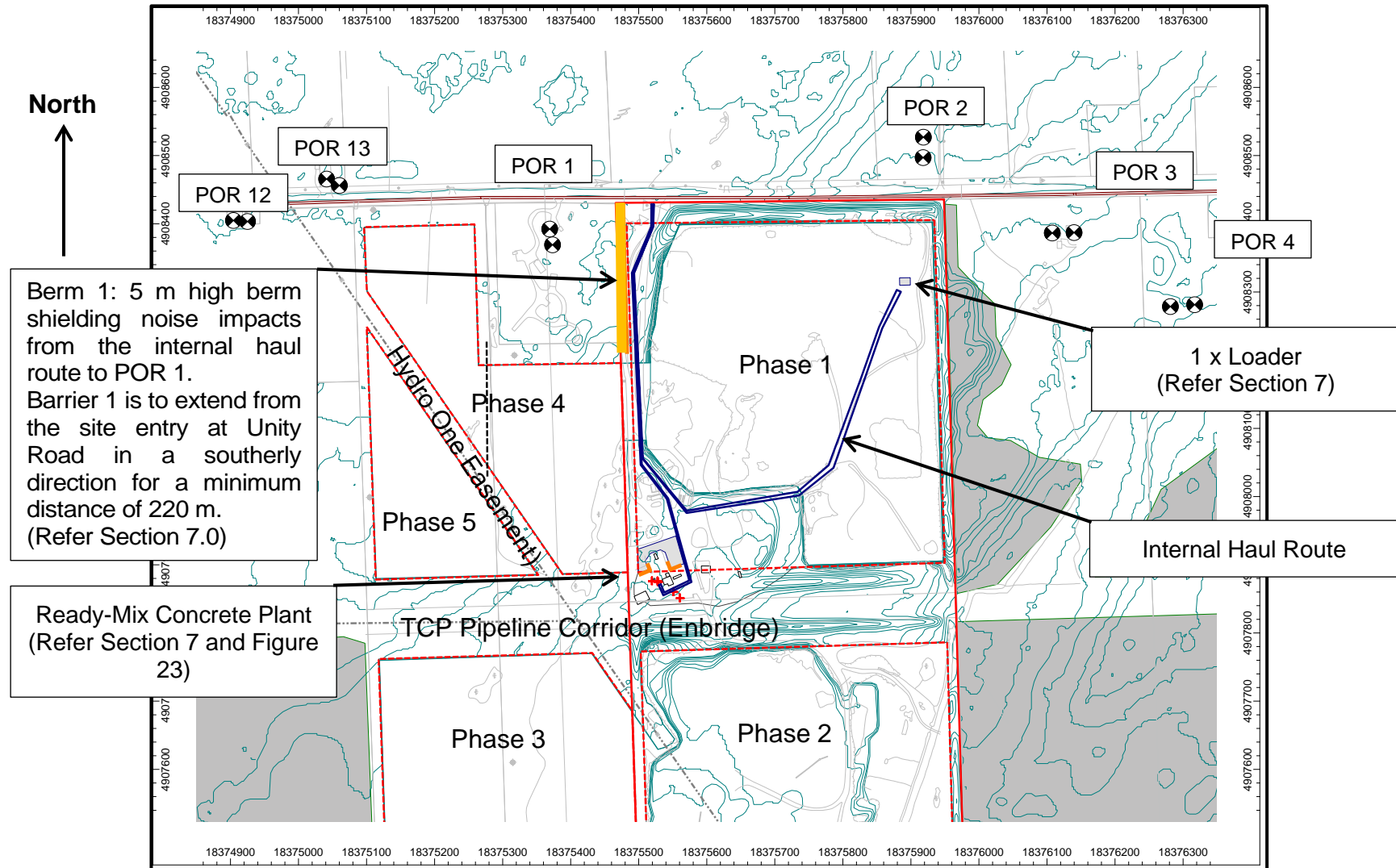
Figure 17: Scenario 8: Worst Case, Existing Quarry, RMC Plant in operation concurrently with loading and hauling operations in Phase 1 (Day, Evening or Night)
