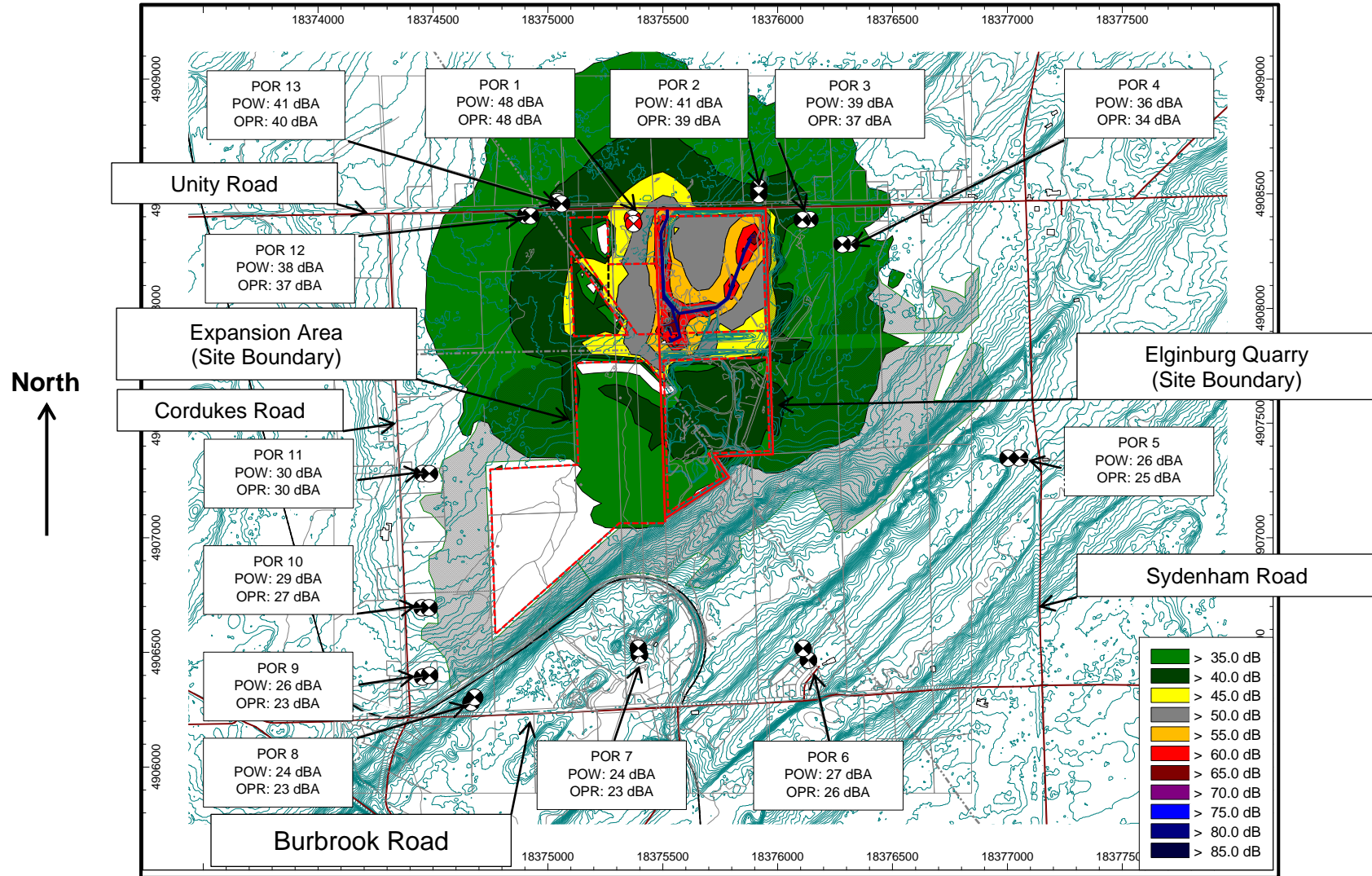
Figure 18.1: Scenario 8: Worst Case – Noise Contours, Night: (Noise levels at 4.5 m) – Before Mitigation
