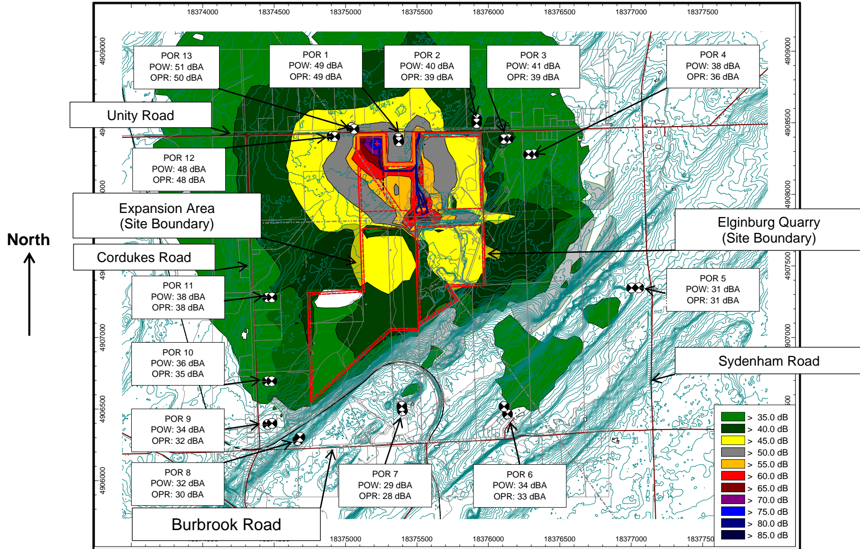
Figure 10.2: Scenario 4: Worst Case – Noise Contours, Day Only: (Noise levels at 4.5 m) – After Mitigation
