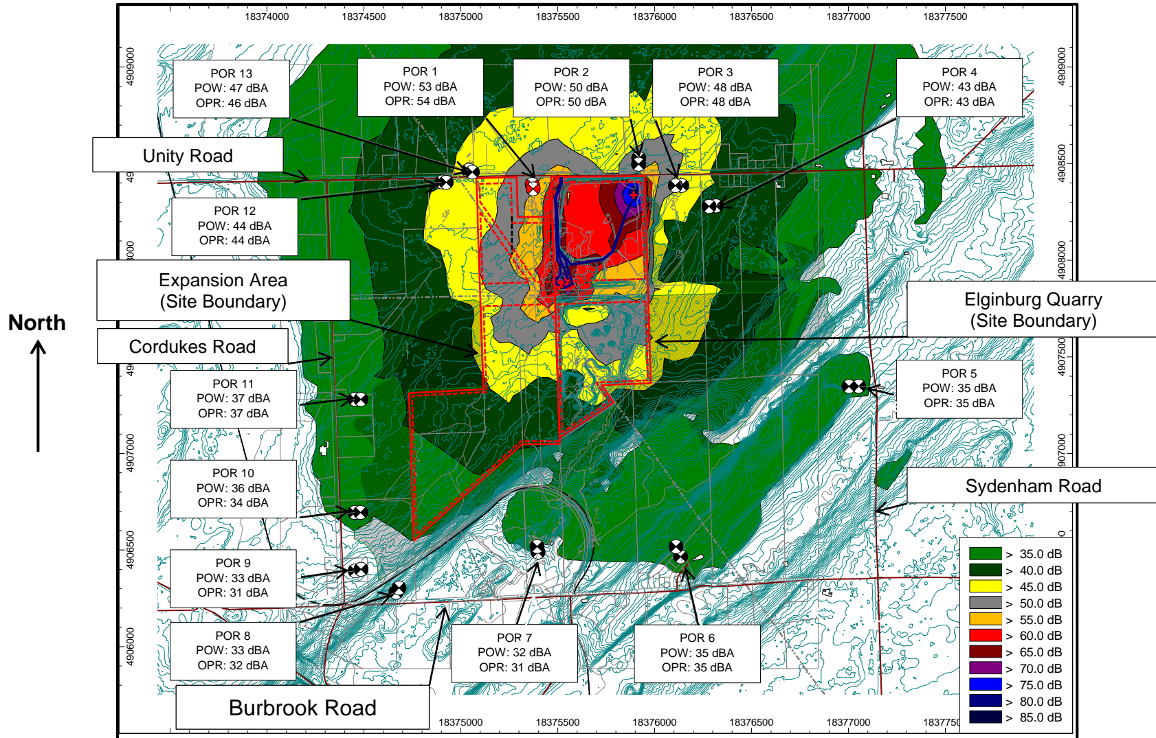
Figure 4.1: Scenario 1: Worst Case – Noise Contours, Day Only: (Noise levels at 4.5 m) – Before Mitigation
