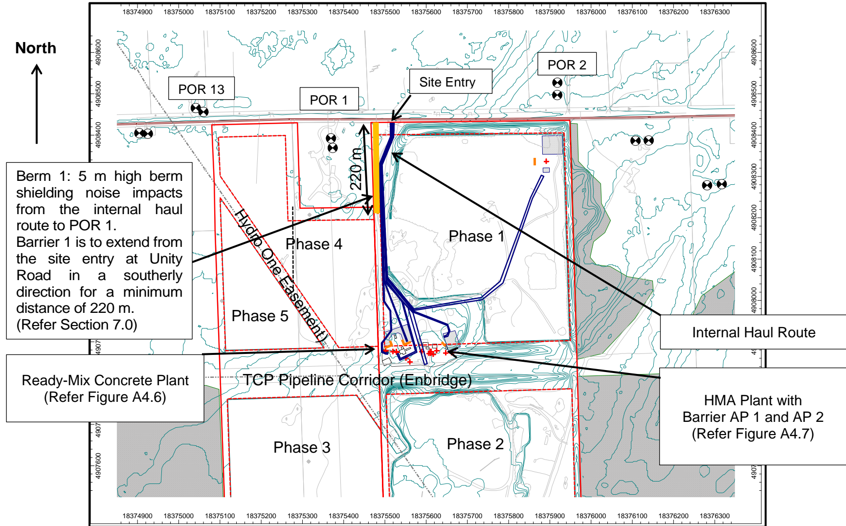
Figure A4.2 Noise Barrier Details – Expansion Area - Phase 4 and Phase 5
