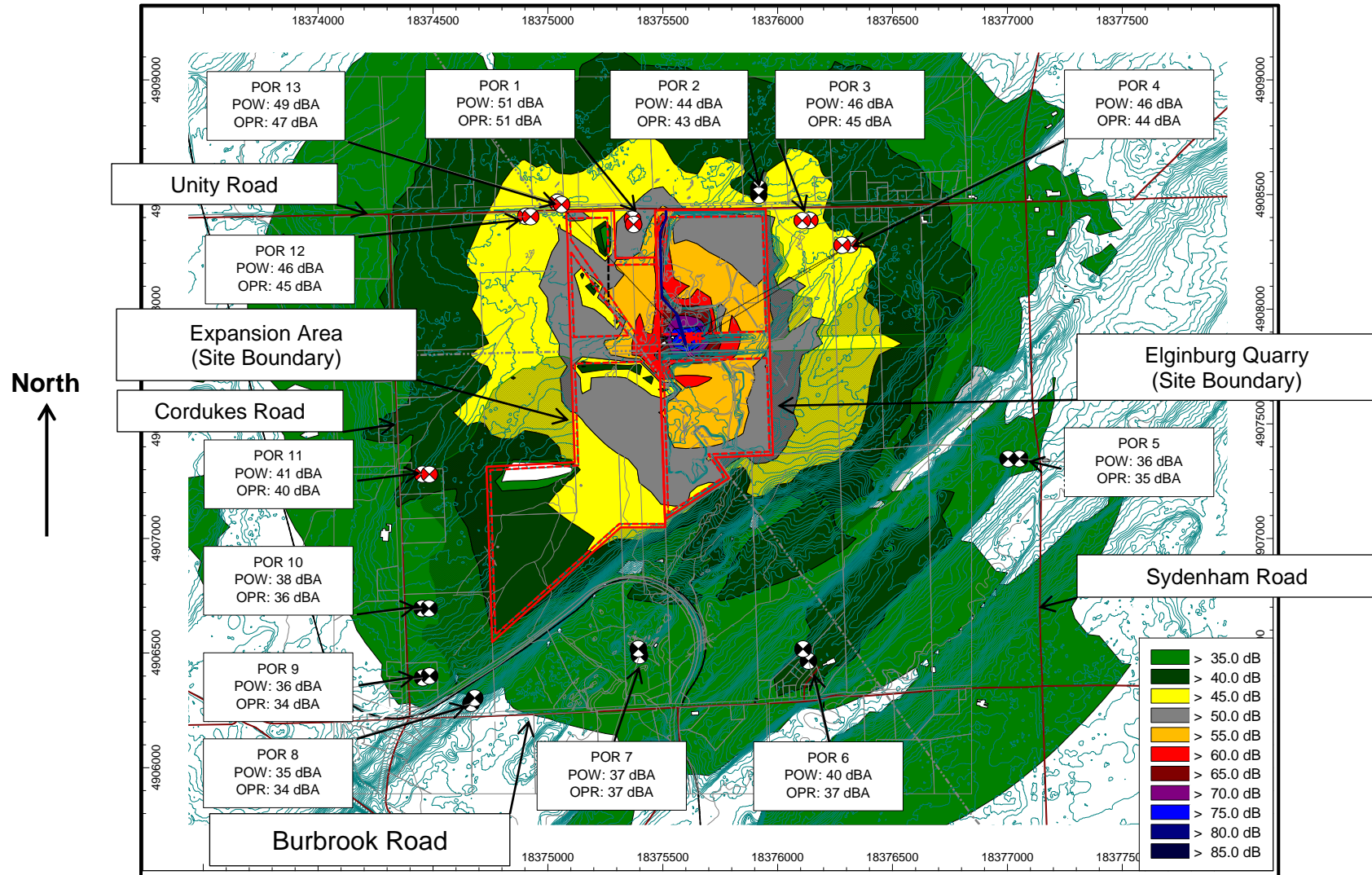
Figure 22.1: Scenario 10: Worst Case – Noise Contours, Night: (Noise levels at 4.5 m) – Before Mitigation
