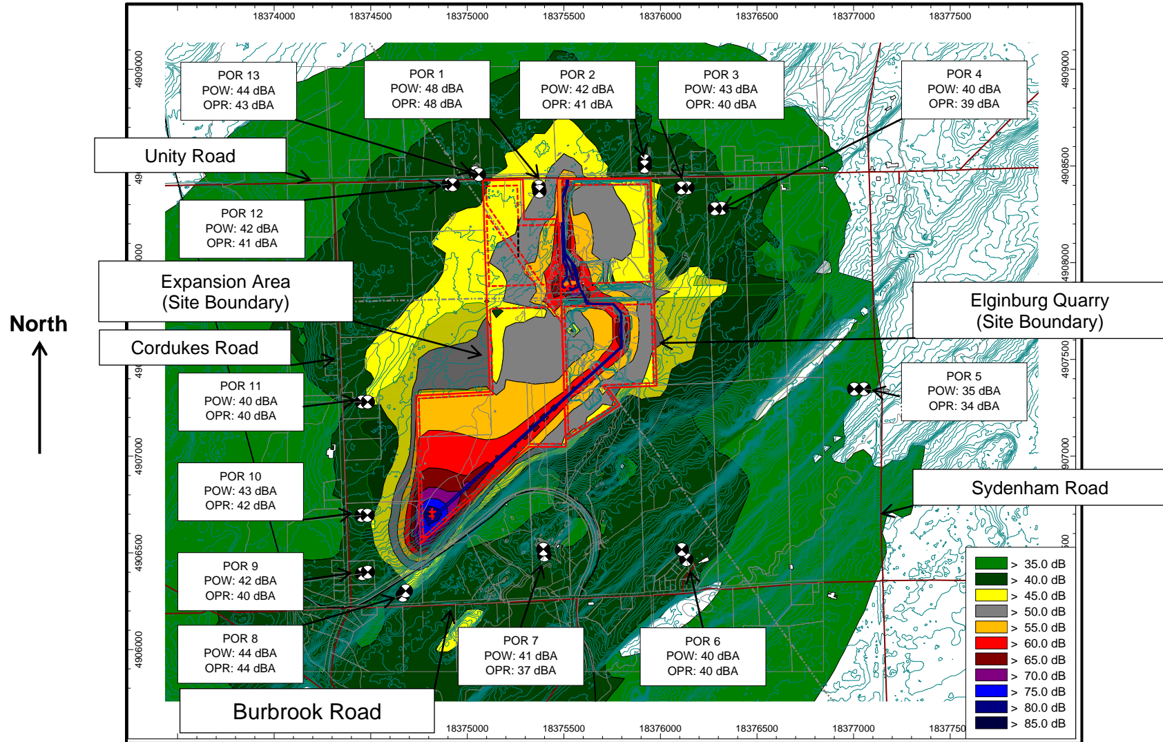
Figure 8.2: Scenario 3: Worst Case – Noise Contours, Day Only: (Noise levels at 4.5 m) – After Mitigation
