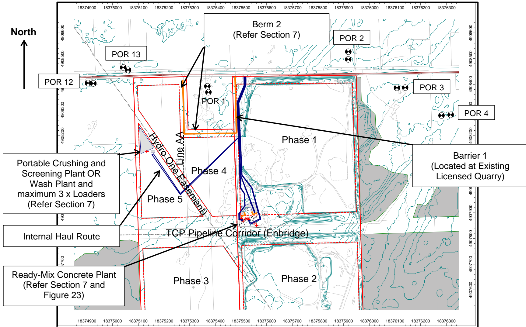
Figure 11: Scenario 5: Worst Case, Expansion Area, RMC Plant in operation concurrently with extraction in Phase 5, Asphalt Plant not in operation (Day only)
