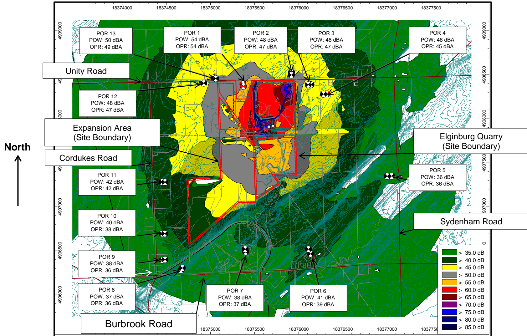
Figure 14.1: Scenario 6: Worst Case – Noise Contours, Day Only: (Noise levels at 4.5 m) – Before Mitigation
