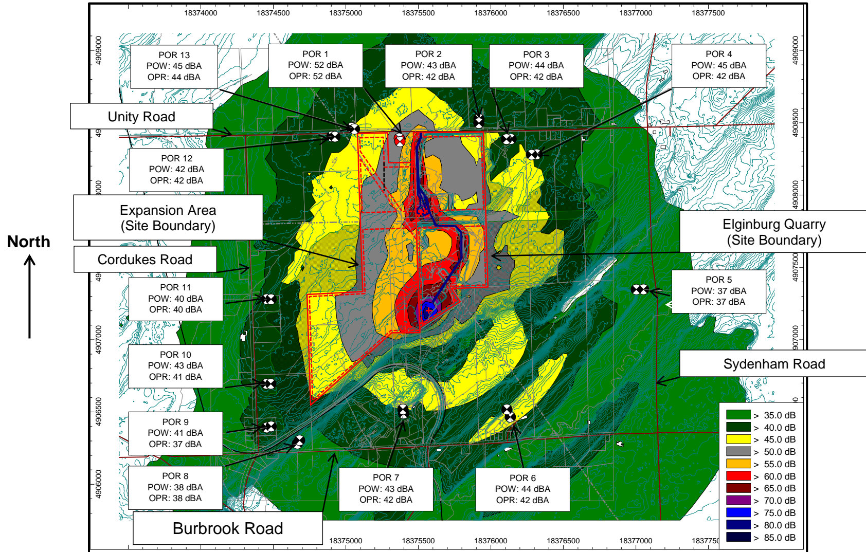
Figure 6.1: Scenario 2: Worst Case – Noise Contours, Day Only: (Noise levels at 4.5 m) – Before Mitigation
