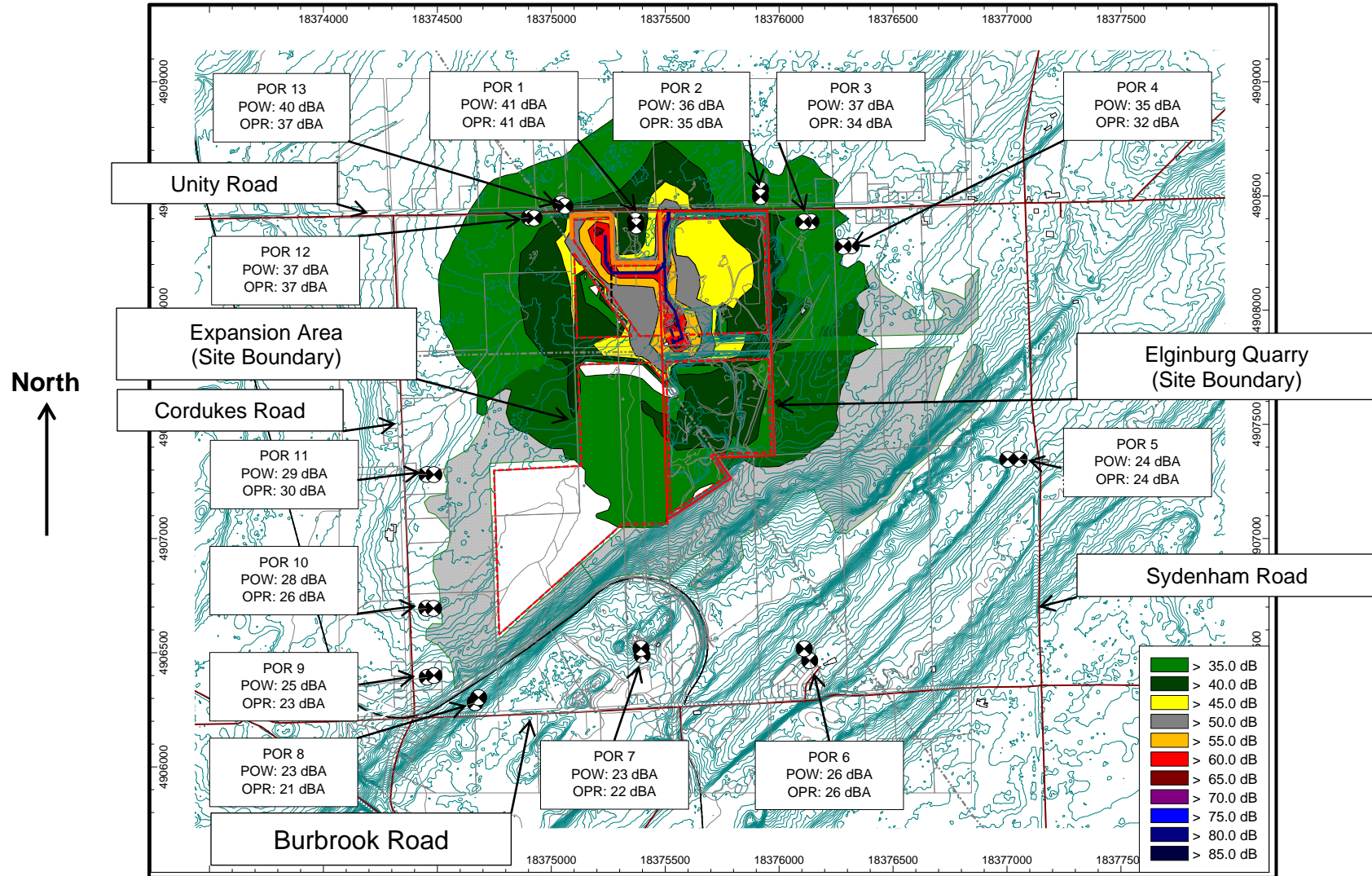
Figure 20.2: Scenario 9: Worst Case – Noise Contours, Night: (Noise levels at 4.5 m) – After Mitigation
