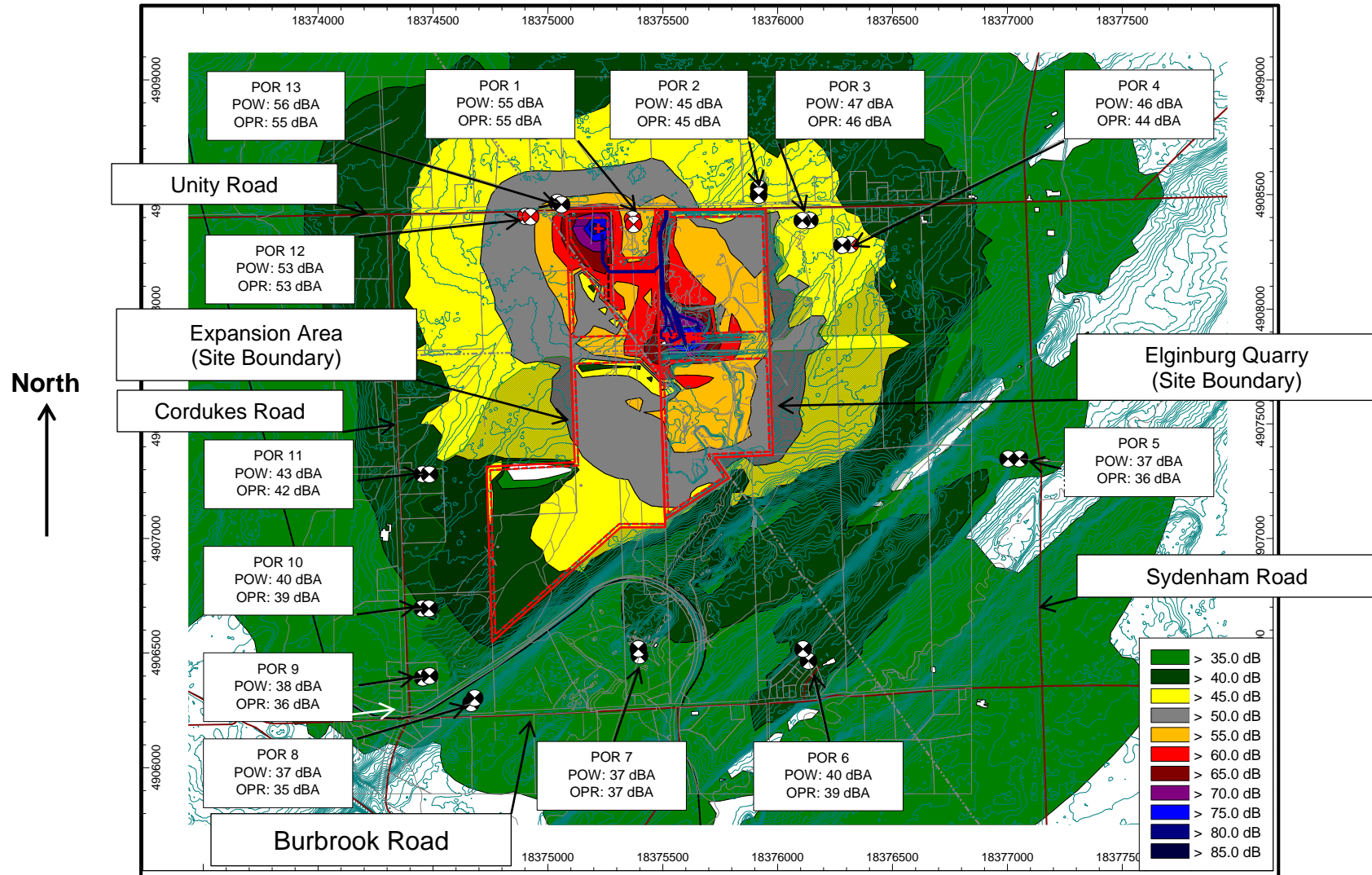
Figure 16.1: Scenario 7: Worst Case – Noise Contours, Day: (Noise levels at 4.5 m) – Before Mitigation
