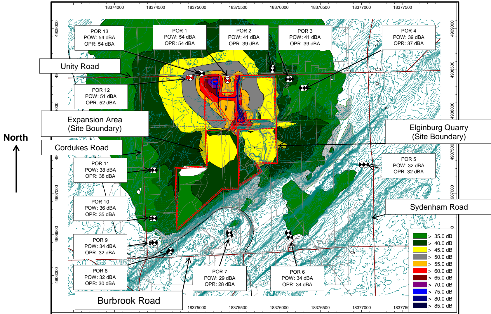
Figure 10.1: Scenario 4: Worst Case – Noise Contours, Day Only: (Noise levels at 4.5 m) – Before Mitigation
