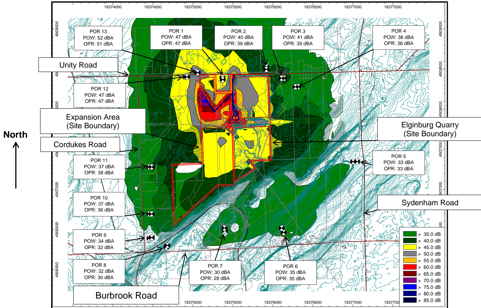
Figure 12.2: Scenario 5: Worst Case – Noise Contours, Day Only: (Noise levels at 4.5 m) – After Mitigation
