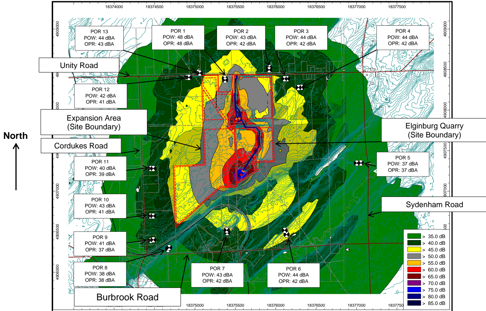
Figure 6.2: Scenario 2: Worst Case – Noise Contours, Day Only: (Noise levels at 4.5 m) – After Mitigation
