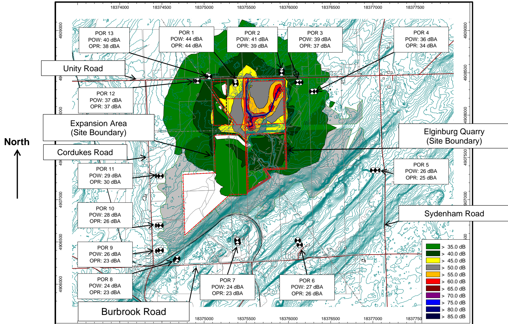
Figure 18.2: Scenario 8: Worst Case – Noise Contours, Night: (Noise levels at 4.5 m) – After Mitigation
