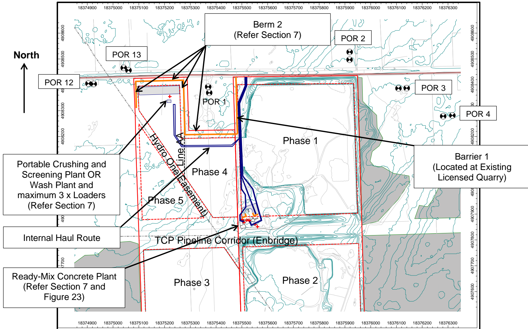
Figure 9: Scenario 4: Worst Case, Expansion Area, RMC Plant in operation concurrently with extraction in Phase 4, Asphalt Plant not in operation (Day only)
