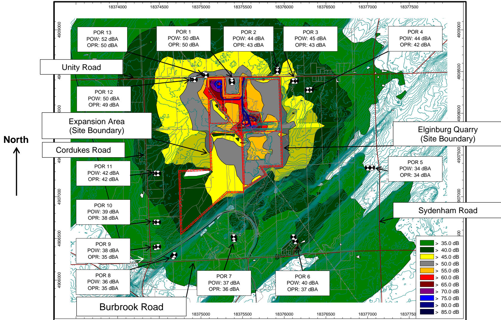
Figure 16.2: Scenario 7: Worst Case – Noise Contours, Day: (Noise levels at 4.5 m) – After Mitigation
