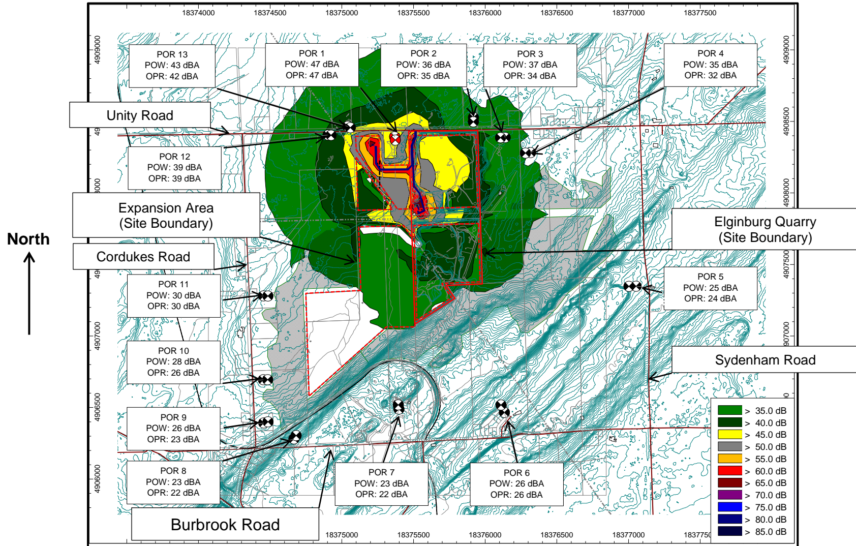
Figure 20.1: Scenario 9: Worst Case – Noise Contours, Night: (Noise levels at 4.5 m) – Before Mitigation
