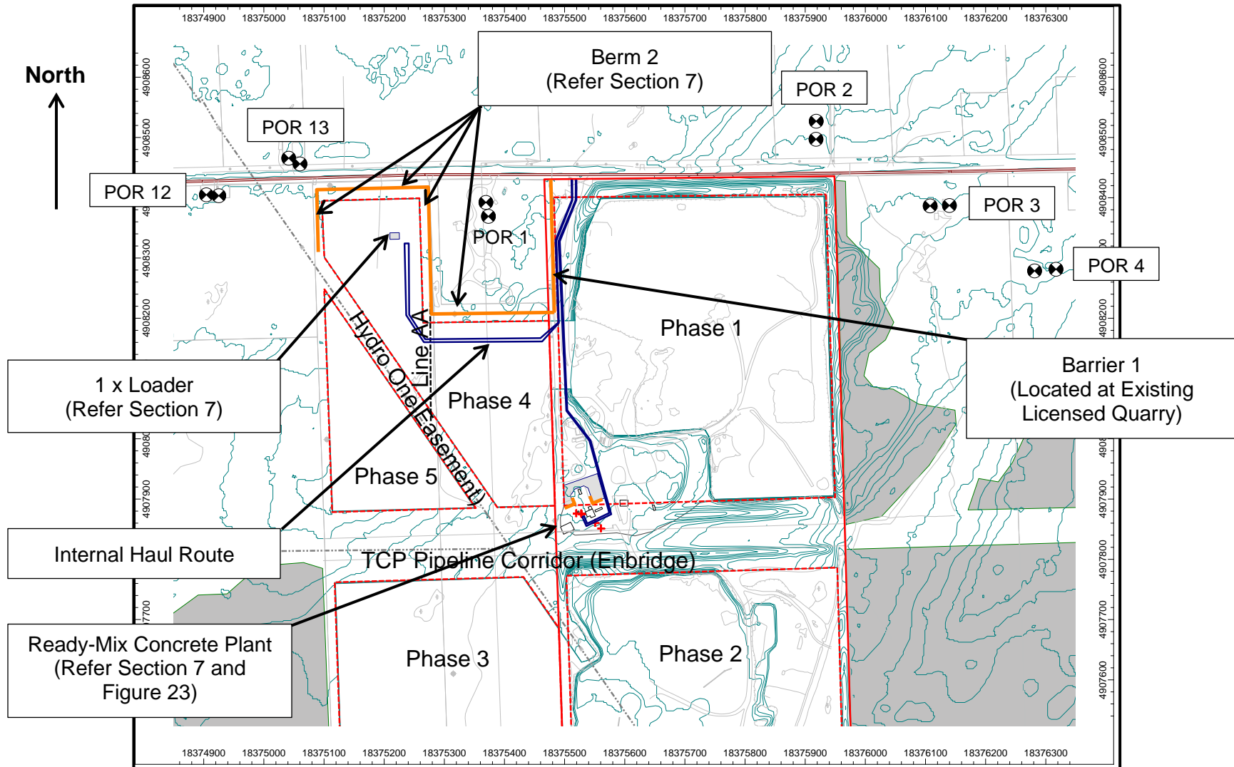
Figure 19: Scenario 9: Worst Case, Expansion Area, RMC Plant in operation concurrently with loading and hauling operations in Phase 4 (Day, Evening or Night)
