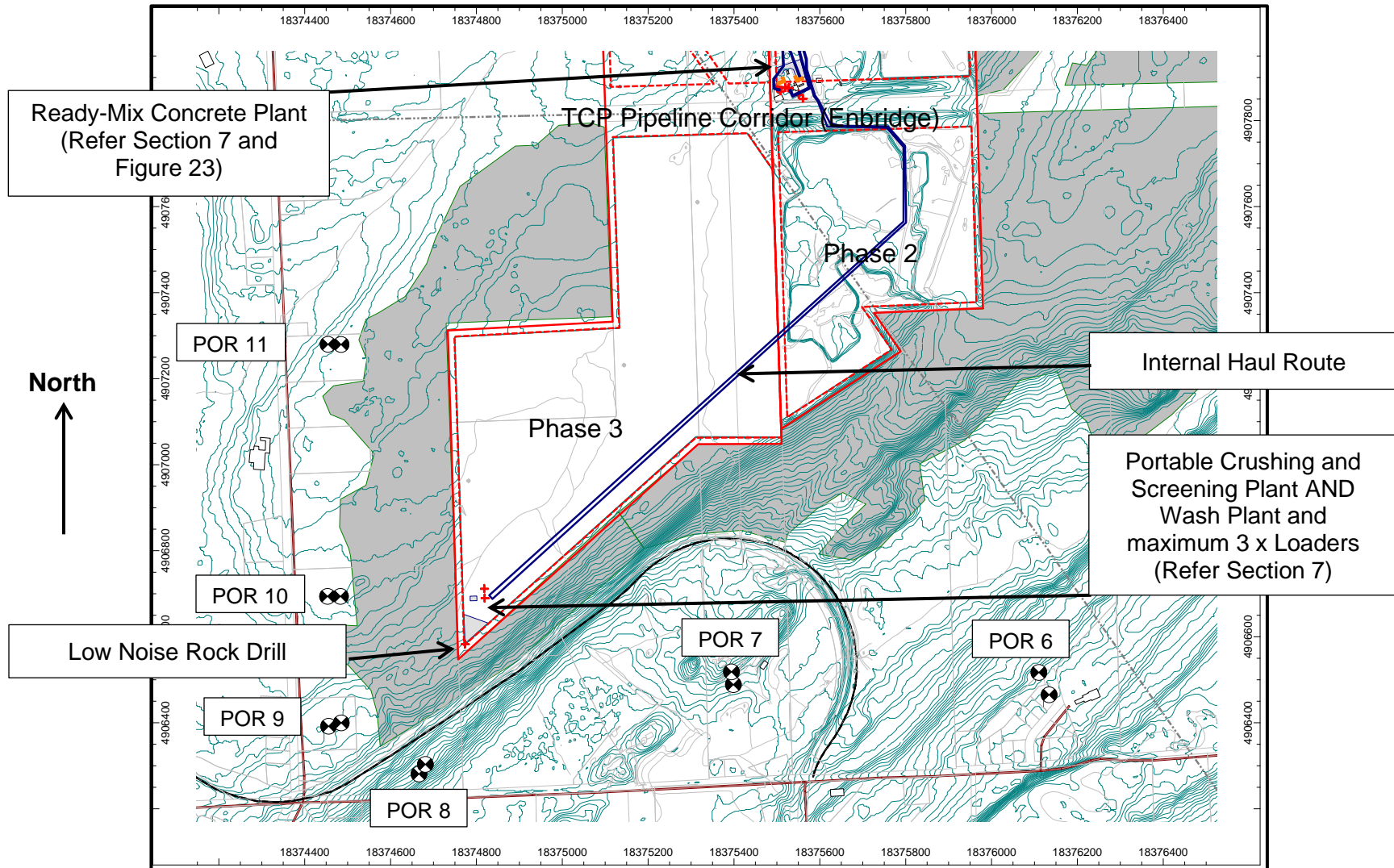
Figure 7: Scenario 3: Worst Case, Expansion Area, RMC Plant in operation concurrently with extraction in Phase 3, Asphalt Plant not in operation (Day only)
