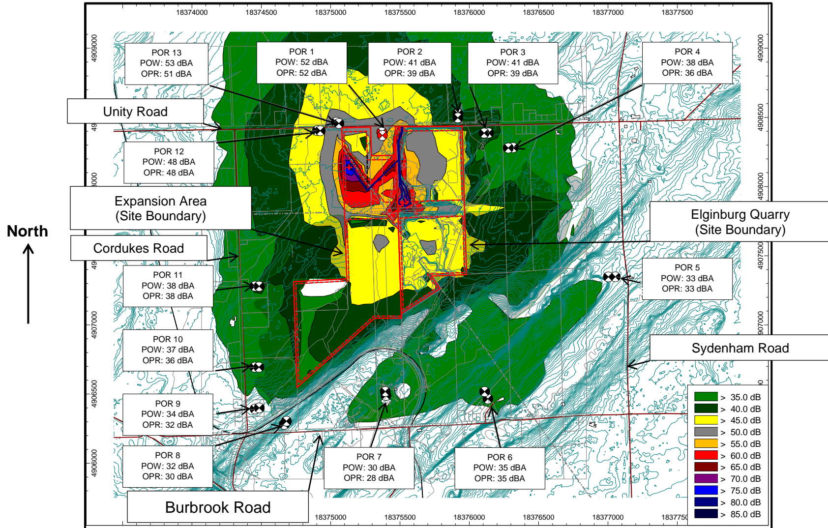
Figure 12.1: Scenario 5: Worst Case – Noise Contours, Day Only: (Noise levels at 4.5 m) – Before Mitigation
