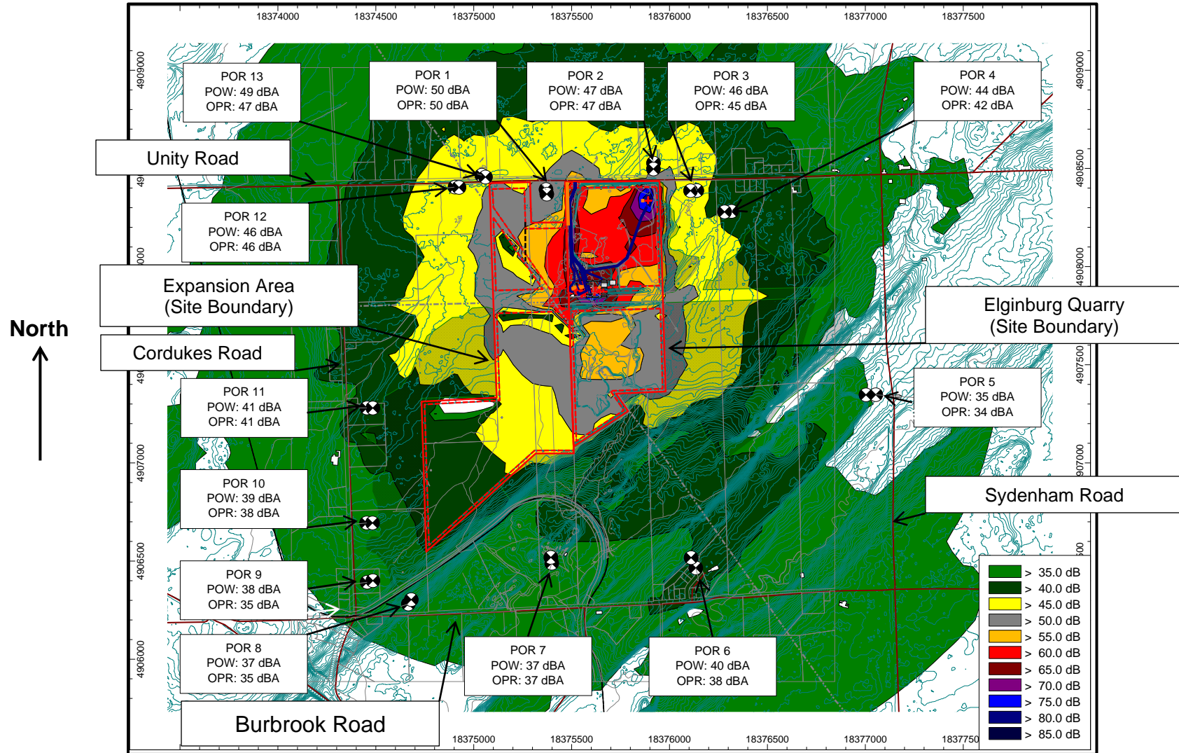
Figure 14.2: Scenario 6: Worst Case – Noise Contours, Day Only: (Noise levels at 4.5 m) – After Mitigation
