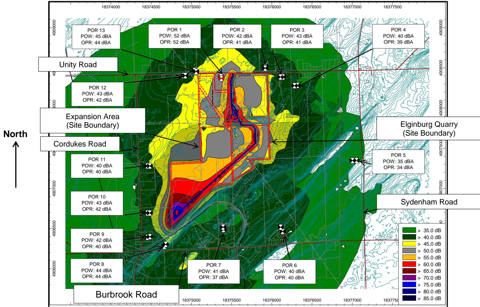
Figure 8.1: Scenario 3: Worst Case – Noise Contours, Day Only: (Noise levels at 4.5 m) – Before Mitigation
